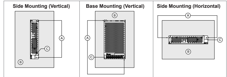
Fig. 2. Mounting Orientation
