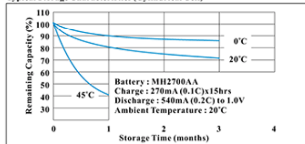
Typical Storage Characteristics (Cylindrical Cell)
