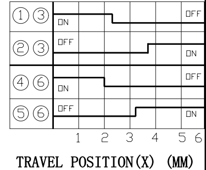
TIME LAG DIAGRAM
