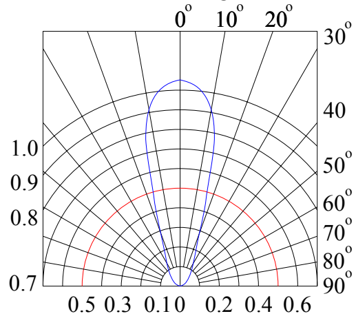
Radiation Diagram
